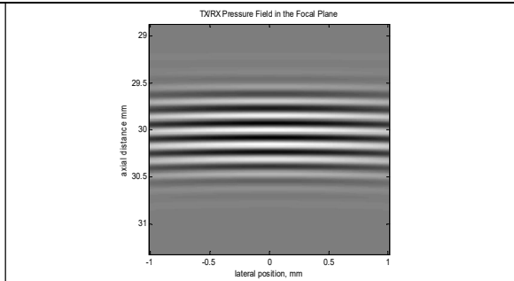
Fig.(e)TX/RX Field image
