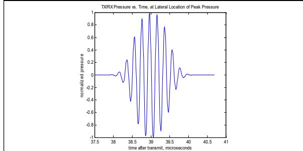
Fig.(f)TX/RX Axial waveform
