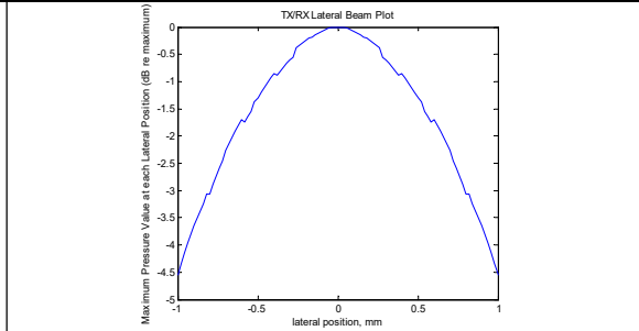
Fig.(g)TX/RX Lateral beam-plot
