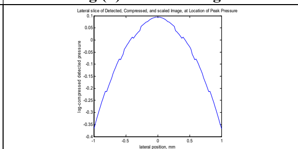
Fig. (m)Detected image lateral slice
